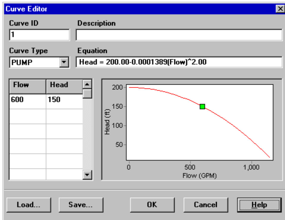
Fig. 3.6: Curve editor.
