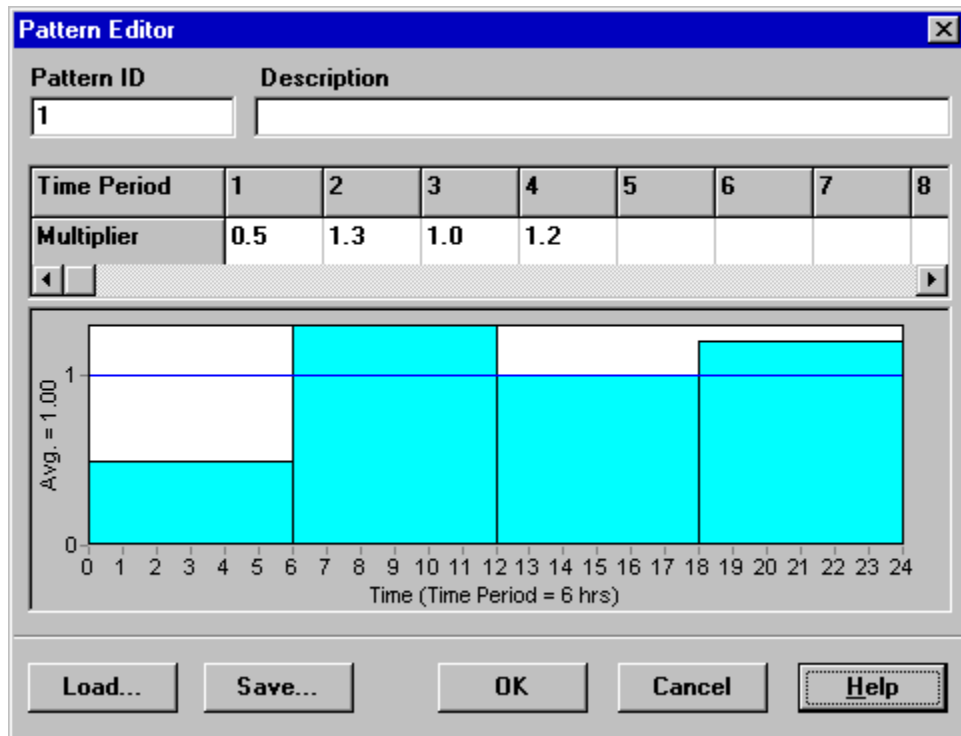
Fig. 7.2: Pattern editor.
