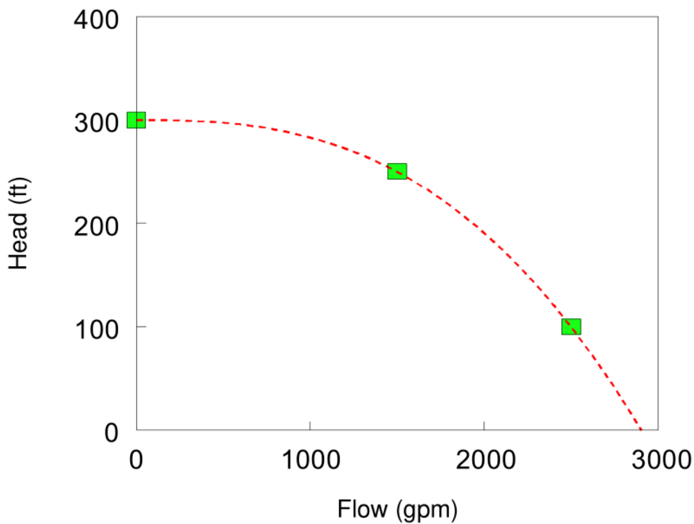
Fig. 4.3: Three-point pump curve.
