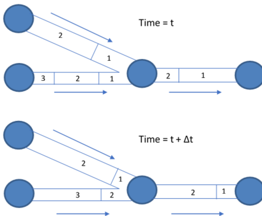
Fig. 14.1: Behavior of segments in the Lagrangian solution method.
