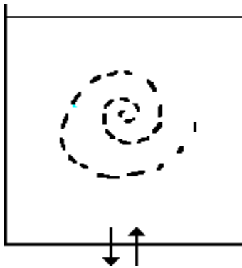
Fig. 4.8: Complete mixing.
