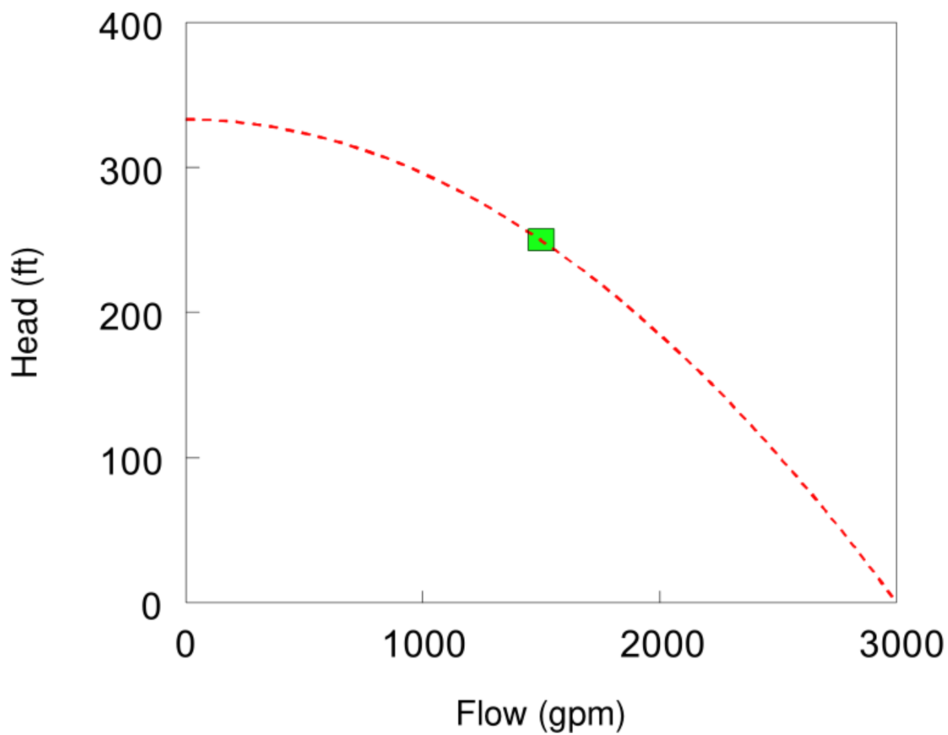
Fig. 4.2: Single-point pump curve.
