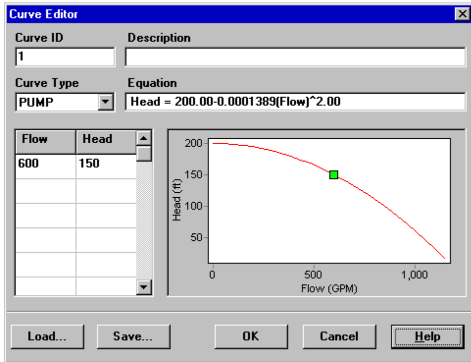
Fig. 7.1: Curve editor.
