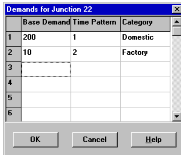
Fig. 7.4: Demand editor.
