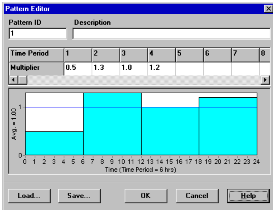
Fig. 3.9: Pattern editor.
