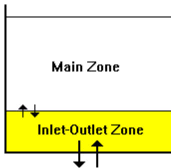
Fig. 4.9: Two-compartment mixing.
