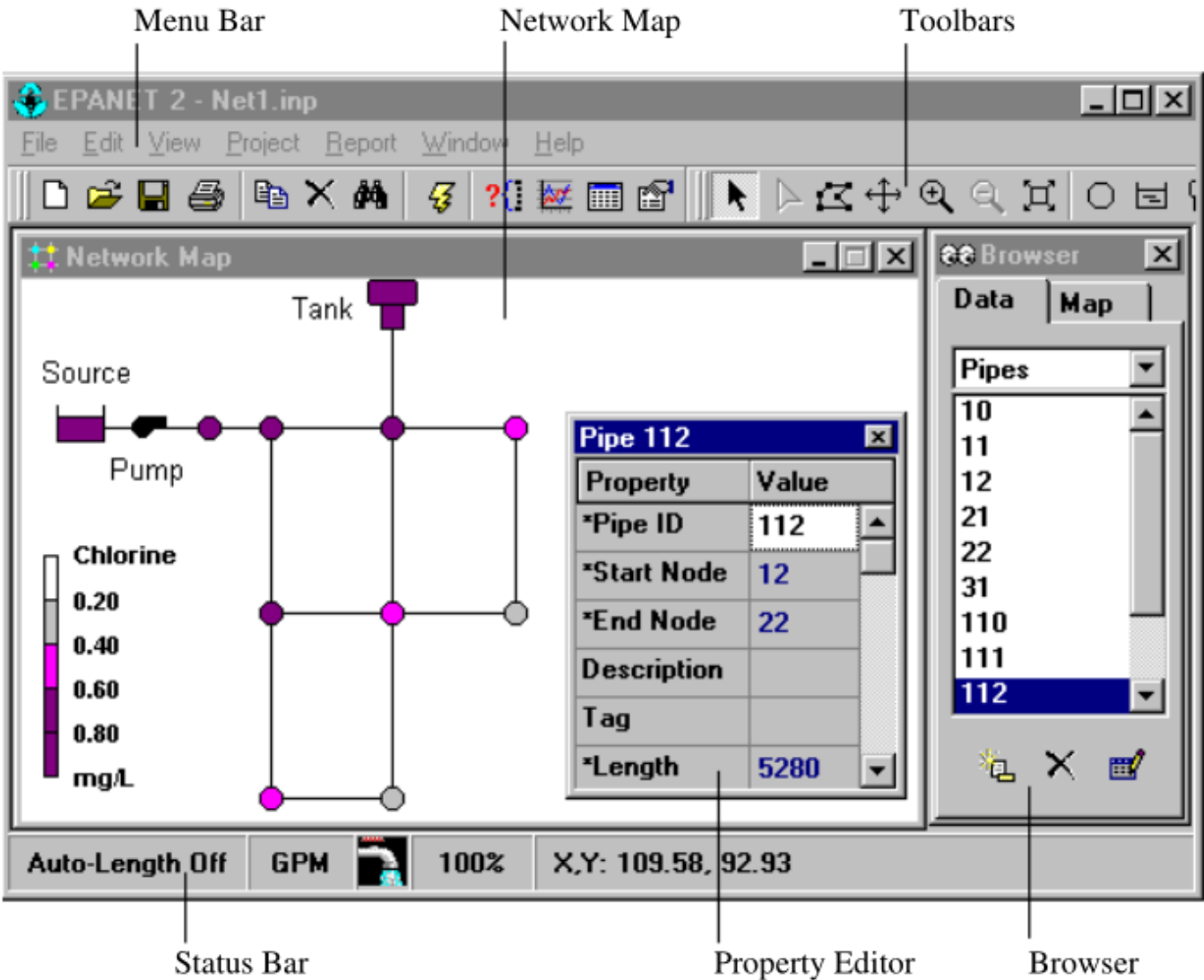
Fig. 5.1: EPANET workspace.
