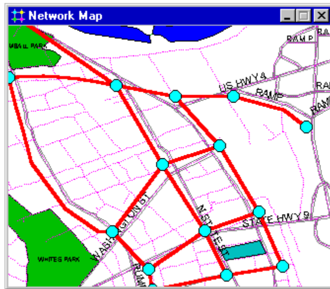
Fig. 8.2: Example backdrop.
