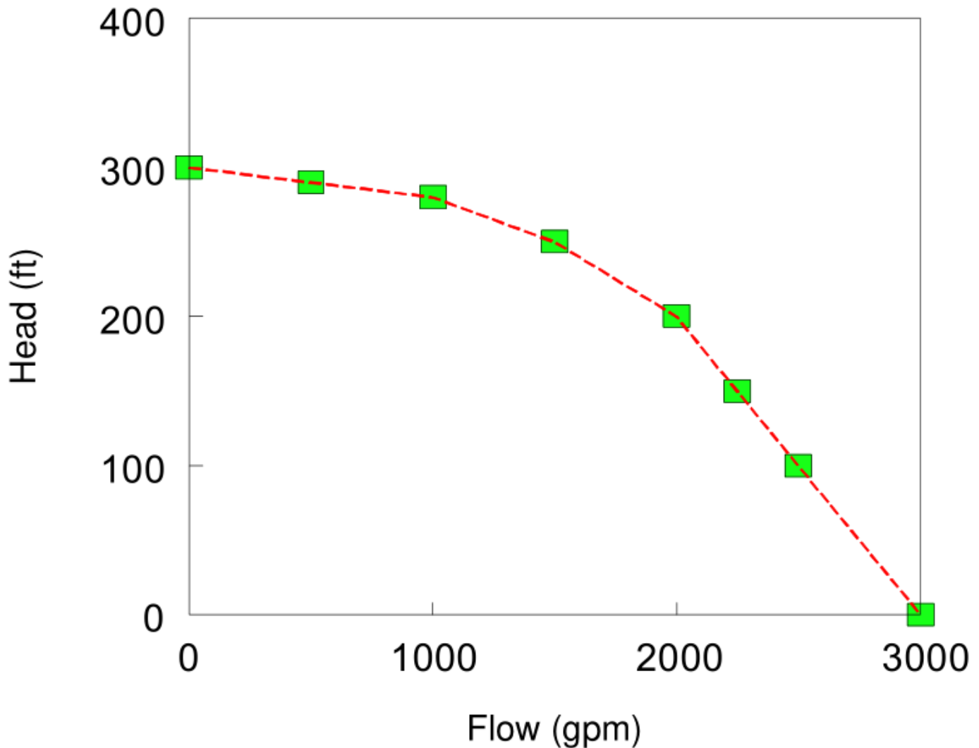
Fig. 4.4: Multi-point pump curve.
