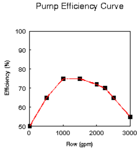
Fig. 4.6: Pump efficiency curve.
