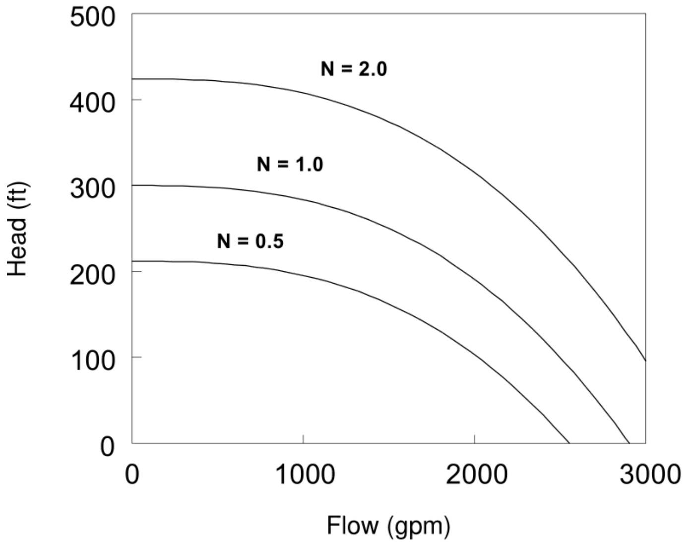
Fig. 4.5: Variable-speed pump curve.
