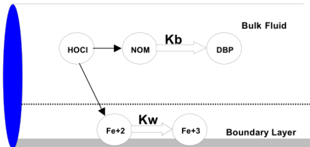
Fig. 4.12: Reaction zones within a pipe.
